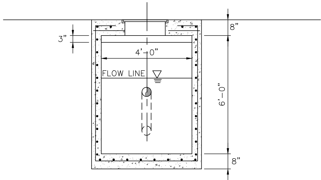
SECTION A
