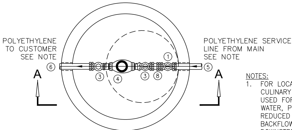
PLAN VIEW
