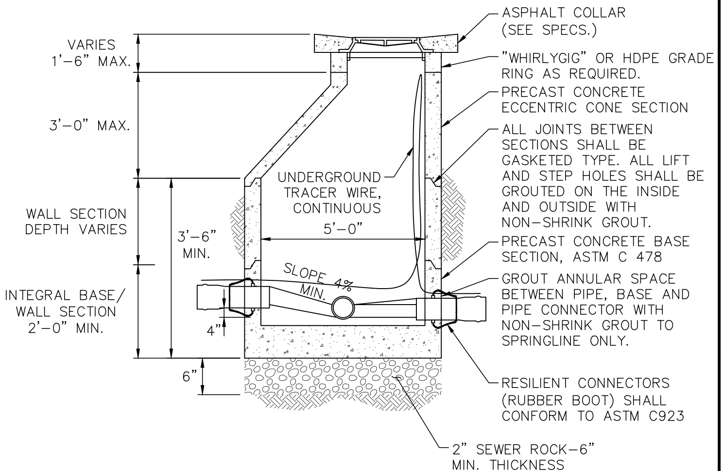
SECTION
