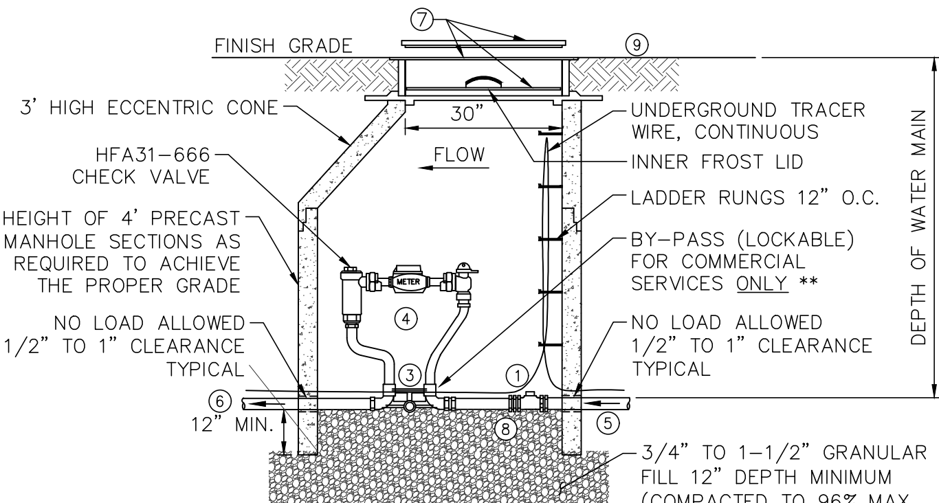
SECTION A
